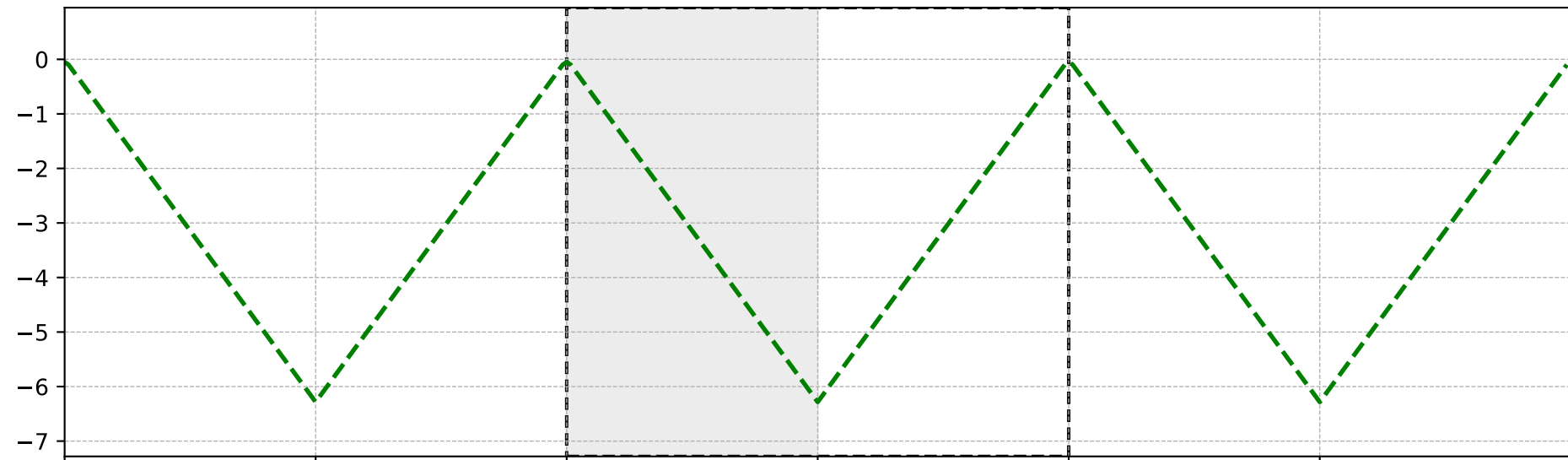
illustration of the convolution calculation at x = 0.60
