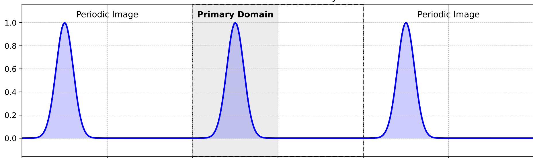
extension of the Green's function g(r) = -2\pi Gr , here G = 1
